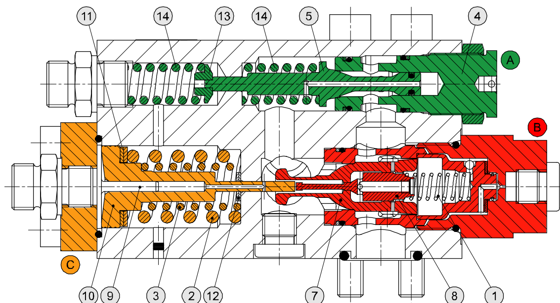
Fig. 1 Sectional view
