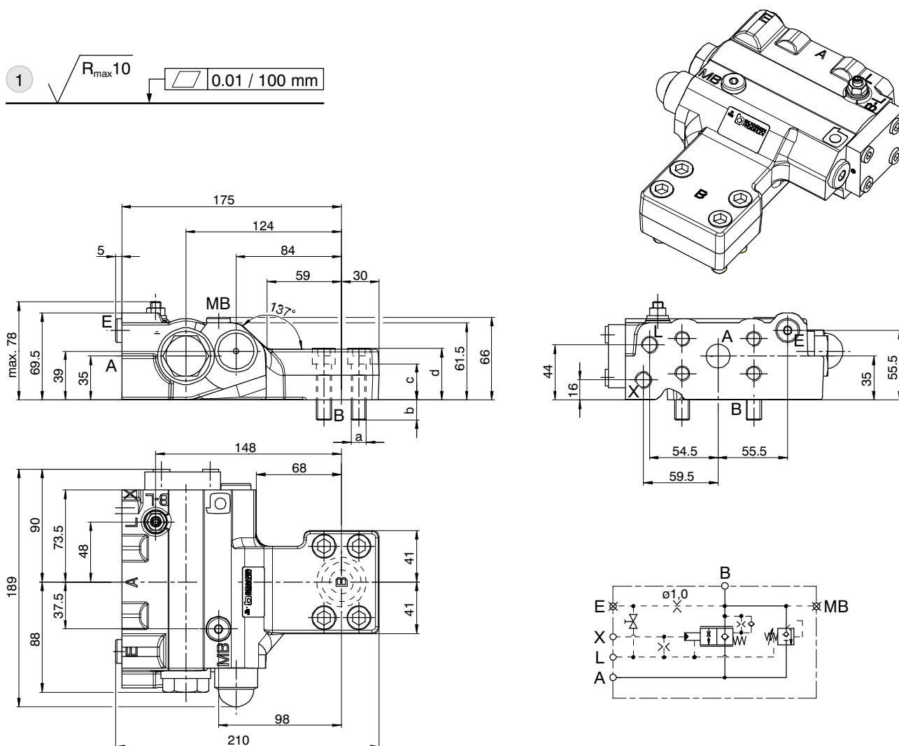
Fig. 5 Dimensions of ESV 16-B-F/ESV 20-B-F
